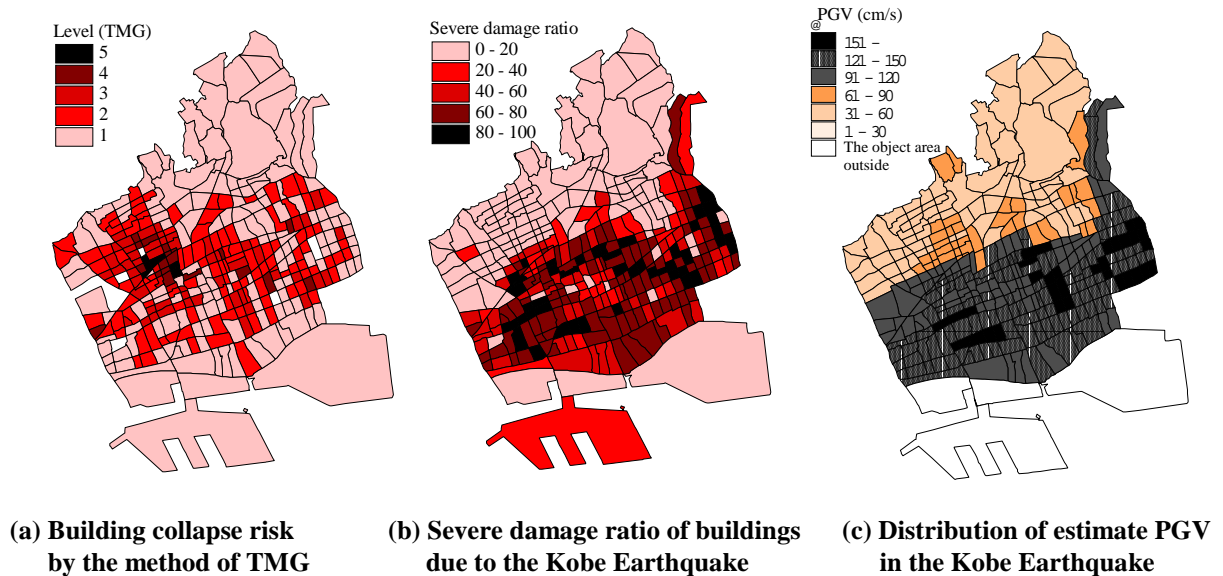
Figure 2: Building collapse risk and actual damage in Nada Ward
