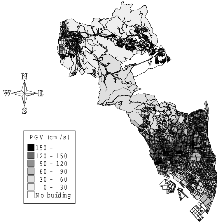
Figure 3: Distribution of estimated PGV in Nishinomiya City
