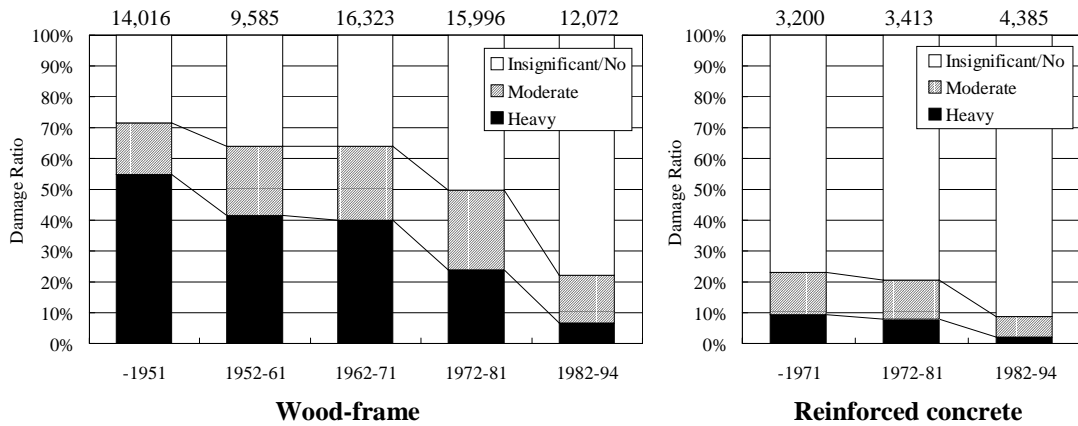
Figure 2: Damage ratio of wood-frame and reinforced concrete buildings in Nishinomiya City with respect to the construction period
