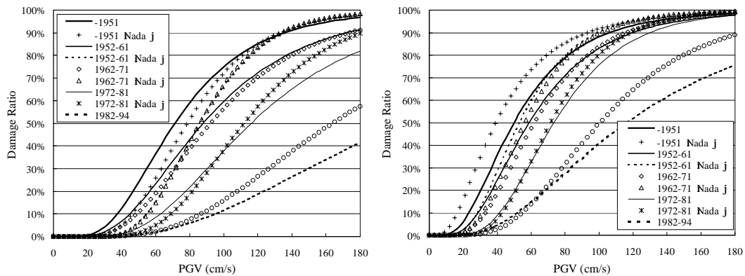
(a) Heavy damage (b) Heavy + Moderate damage Figure 8: Comparison of obtained fragility curves with those for Nada Ward (wood-frame with different construction periods)
