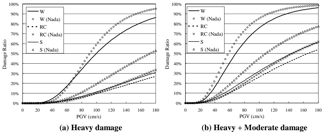
Figure 7: Comparison of obtained fragility curves with those for Nada Ward (different structural types)
