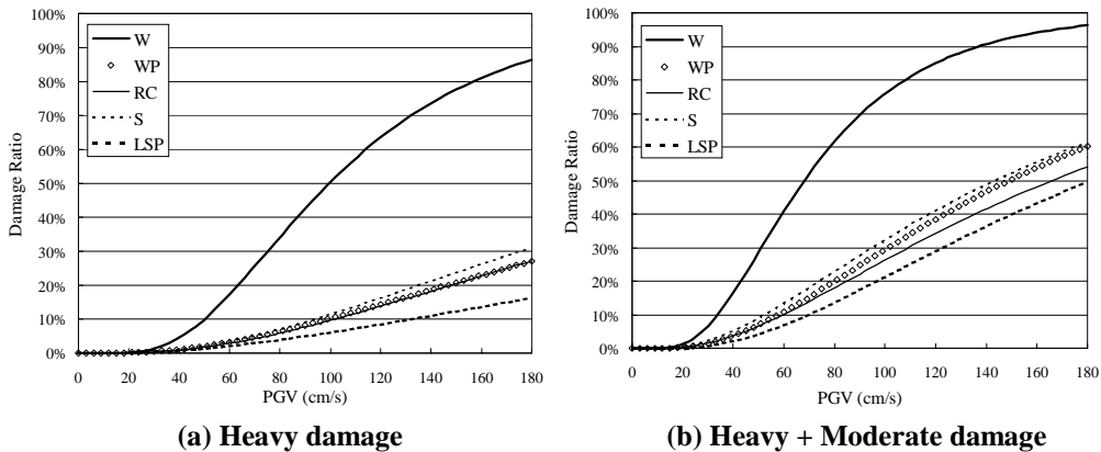
Figure 4: Fragility curves with respect to PGV for different structural types
