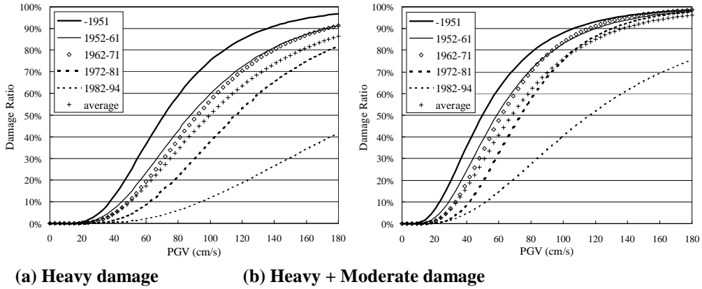
Figure 5: Fragility curves of wood-frame buildings with respect to PGV for different construction periods
