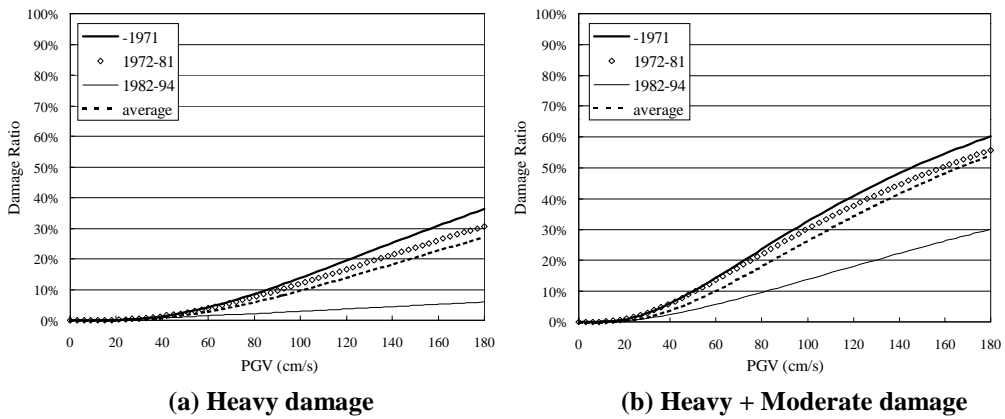
Figure 6: Fragility curves of reinforced concrete buildings with respect to PGV for different construction periods
