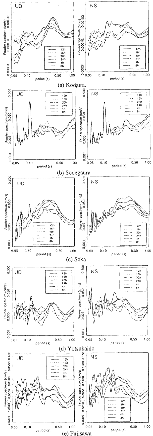
Fig. 3 Fourier spectrum at the five sites
