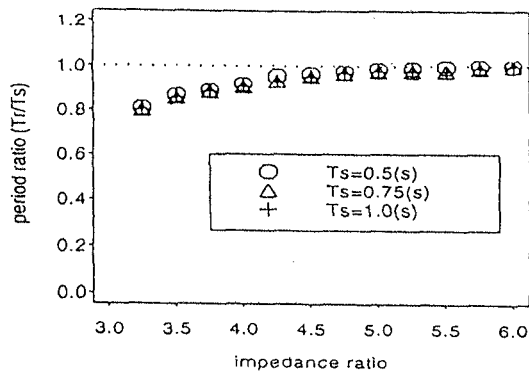
Fig. 6 Relationship between impedance ratio and period ratio ( T_r/T_s ) of Rayleigh and S-waves.
