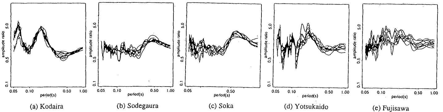
Fig. 4 Fourier spectrum ratio at the five sites.
