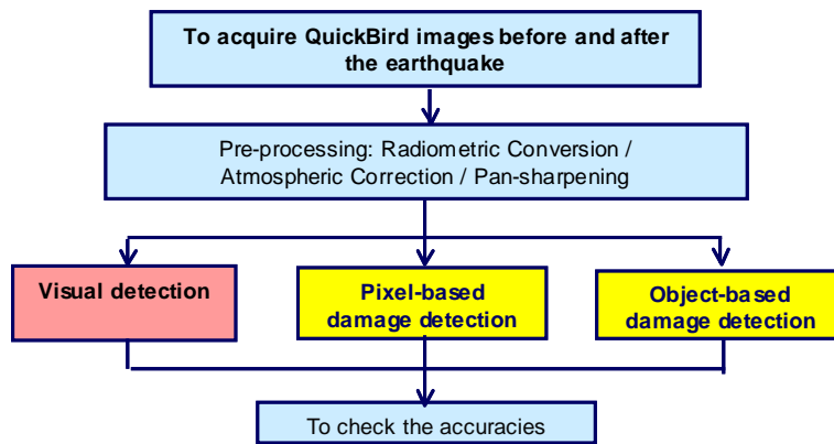
Figure 3. Flowchart of all operations.
