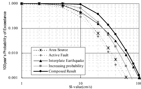
Figure 5. Seismic hazard curve on the base rock( V_s=600\text{m/s} ).
