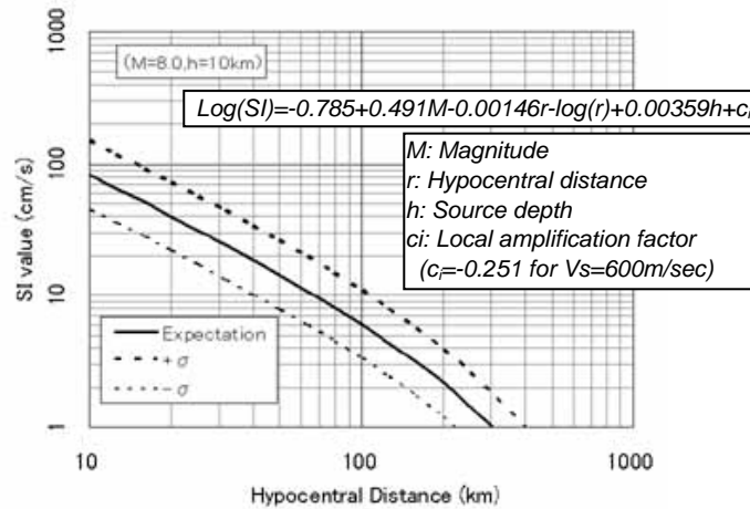
Figure 4. Attenuation function for the SI-value used in the analyses.
