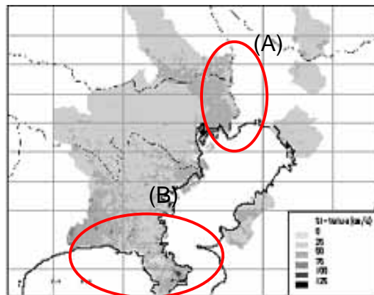
Figure 6. Seismic hazard map on the ground surface (the probability of exceedance in 100 years: 39.5%).
