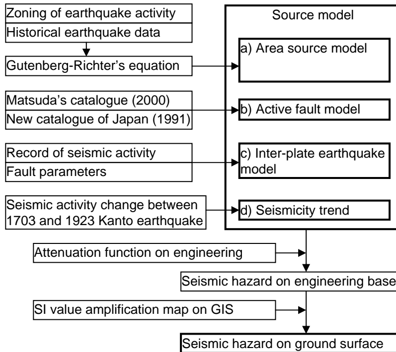
Figure 2. Flowchart of the seismic hazard analysis.
