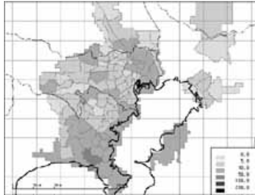
Figure 8. Expected value of breaks for low-pressure pipes in 15-year period.
