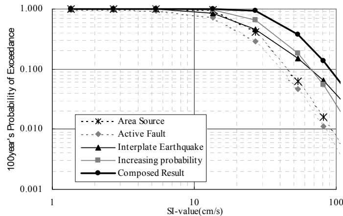
Figure 7. Seismic hazard curves on the ground surface.
