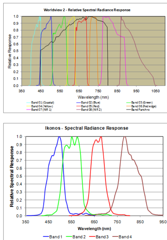
Figure 2. Spectral response comparison between Worldview 2 and Ikonos images.
