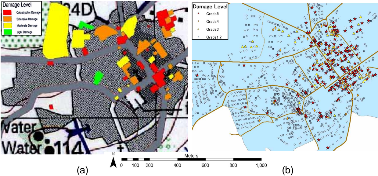
Figure 12. (a) Damage map for Zemmouri evaluated by the United States Government (UN-OCHA, 2003), (b) our detection result
