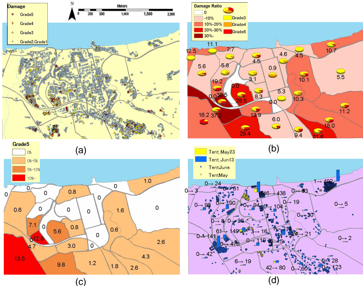
Figure 7. Damage and tent distribution map. (a) total 3,446 buildings classified based on their damage grades, (b) the ratio of damage buildings in each city block, (c) the ratio of Grade5 buildings in each city block, (d) the locations of tents in the two post-event images
