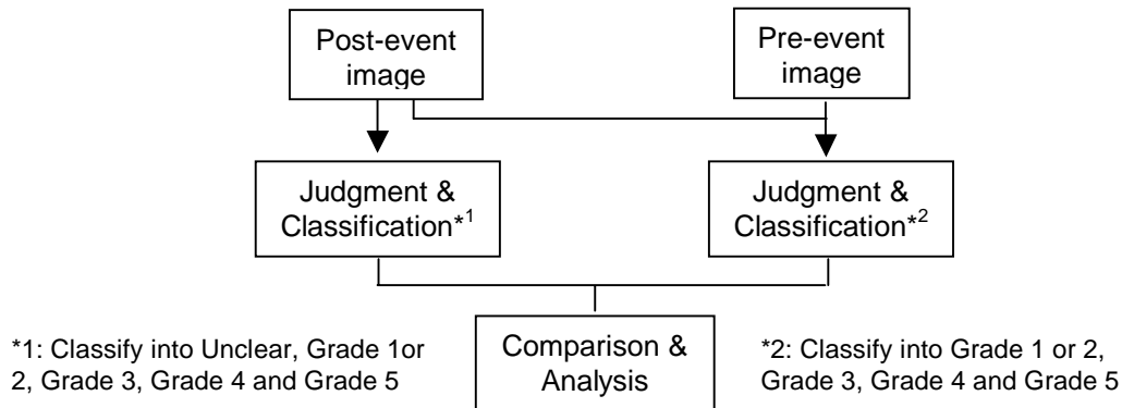
Figure 4. Flowchart to classify building damage
