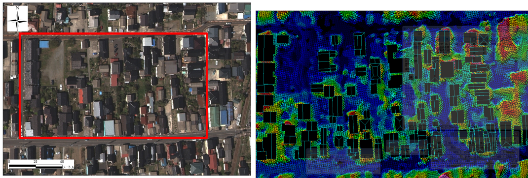
Figure 4. The digital surface model constructed automatically and the breaklines to describe the discontinuities of elevation.
