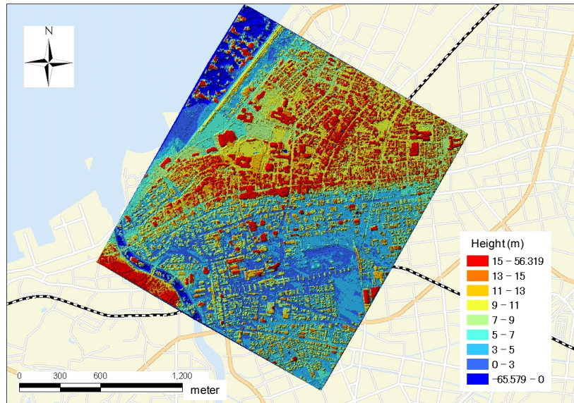
Figure 3. The digital surface model in Kashiwazaki city constructed from the pre-event images.
