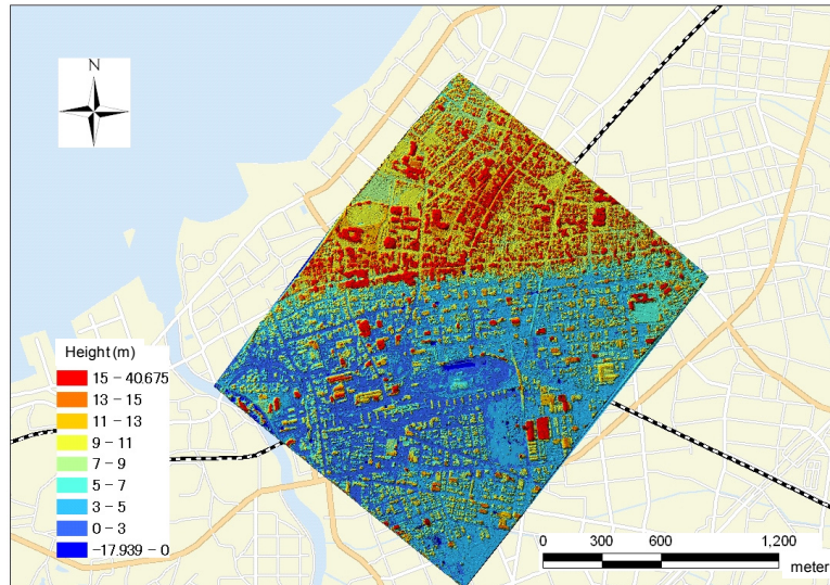
Figure 7. The DSM constructed from the post-event images.
