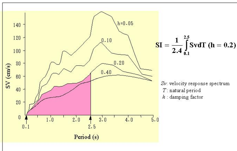
Figure 1. Definition of spectrum intensity SI.
