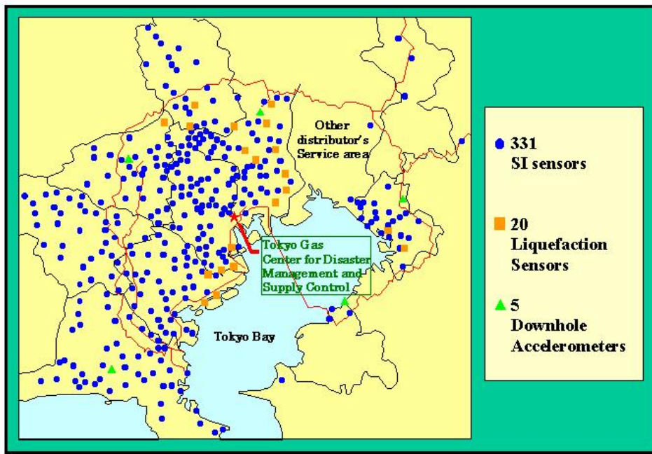
Figure 3. Distribution of seismic sensors of SIGNAL.
