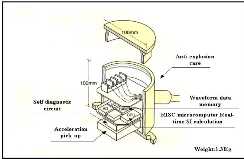
Figure 4. New SI sensor.
