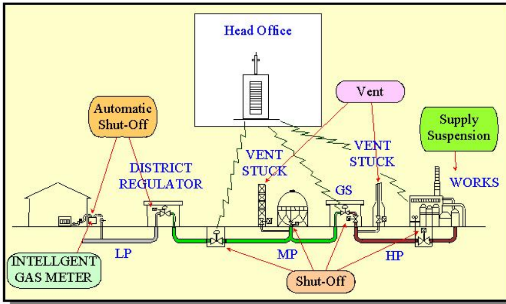
Figure 2. Emergency shutoff systems of natural gas network of Tokyo Gas Co., Ltd.
