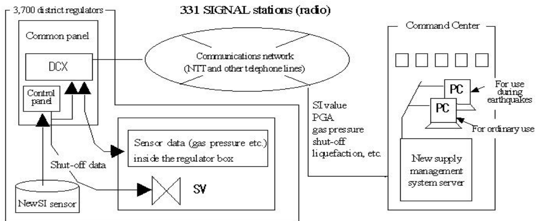
Figure 6. System configuration of SUPREME.
