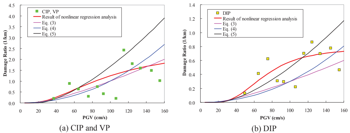
Figure 5: Relationship between results of nonlinear regression analysis and fragility curves for water distribution pipelines.
