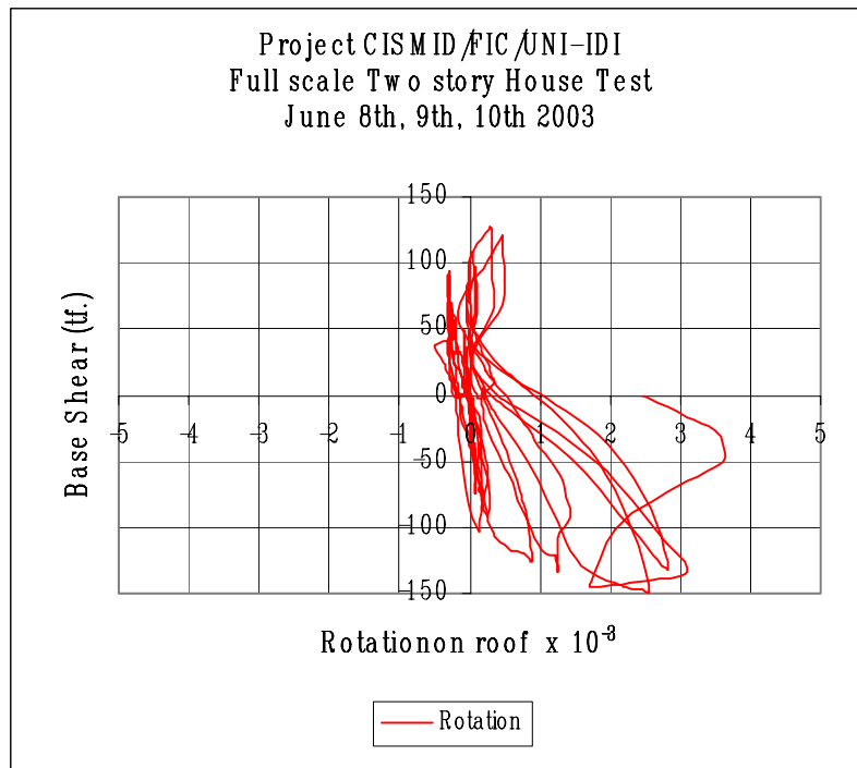
FIGURE 9: measured rotation on roof
