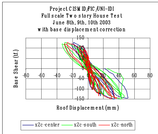
FIGURE 12: Second floor load - displacement corrected
