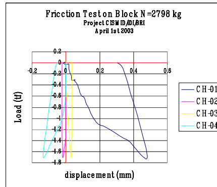
FIGURE 5: Load – displacements on block
