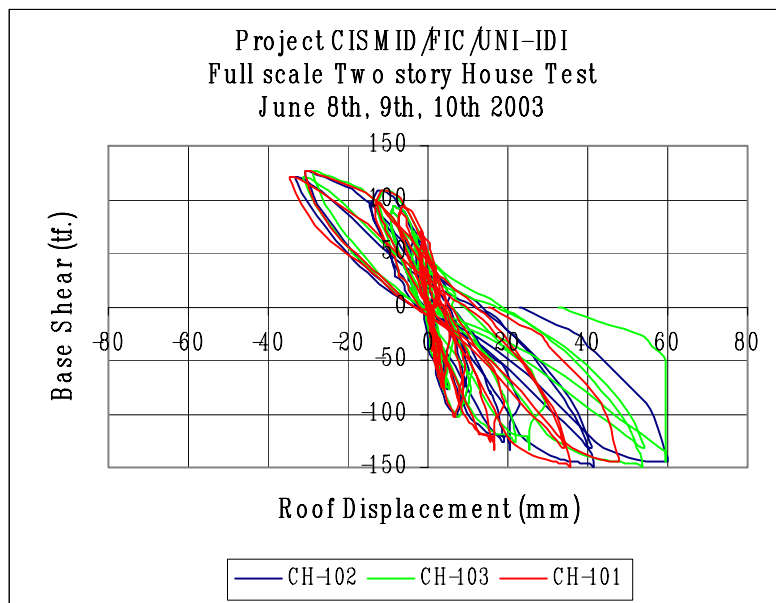
FIGURE 8: First floor displacement history
