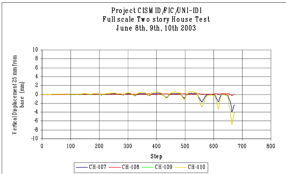
FIGURE 10: Vertical displacement at level 25 mm. from basement
