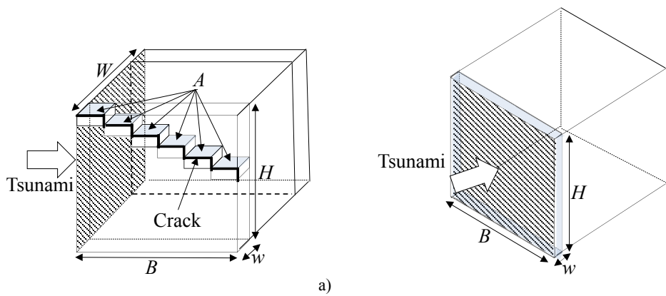
Fig. 4. Relationship between the direction of a tsunami wave and the longitudinal axis of a wall: a) paired walls at right angles to the coastline and b) wall along the coastline.
