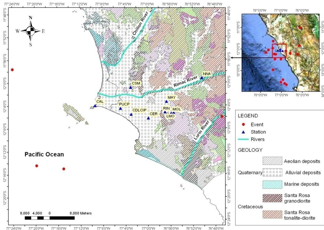
Figure 1 Red circles show the epicenter of events used for this work. Blue triangles represent the stations which are located on the geological map of Lima city (Martinez et al. 1975).
