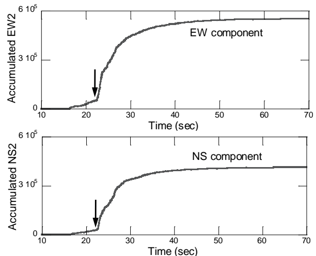
Figure 3. Husid plots to recognize the onset time of S-wave. Black arrows indicate the S-wave onset time (CSM station, seismic event 2008/03/29 12:51).
