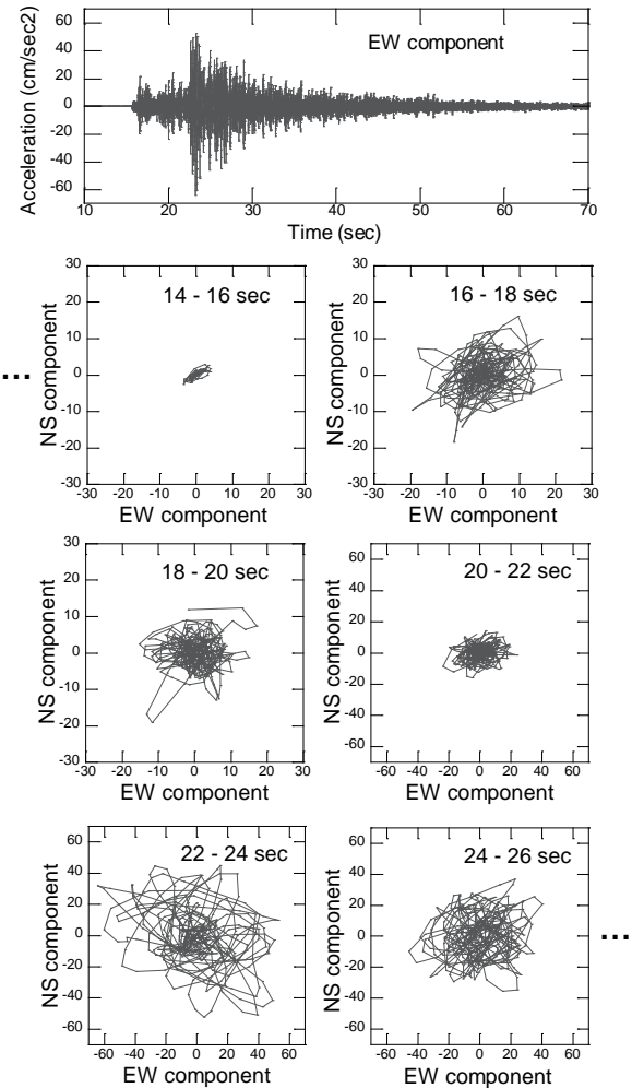
Figure 2. Particle motion plots for two components of motion (CSM station, seismic event 2008/03/29 12:51).
