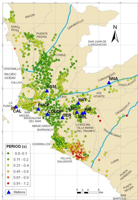
Figure 6. Location of seismic stations over the predominant period distribution map obtained from the H/V spectrum of single-point microtremor measurements (Calderon 2012).
