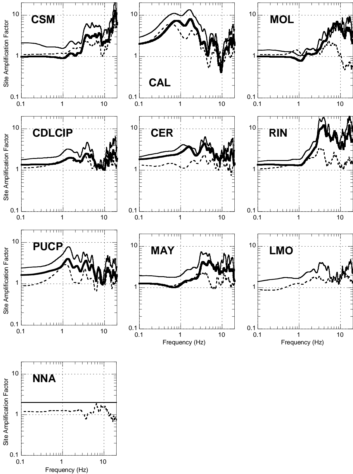
Figure 4. Comparison between spectral ratios from the horizontal components with reference to NNA, the Spectral Inversion Method and the Horizontal-to-Vertical Spectral Ratio. Thick solid lines show the geometrical average of two horizontal spectral ratios. Thin solid lines represent the results obtained by the Spectral Inversion Method. Dotted lines show the geometrical average estimated by applying the HVSR.
