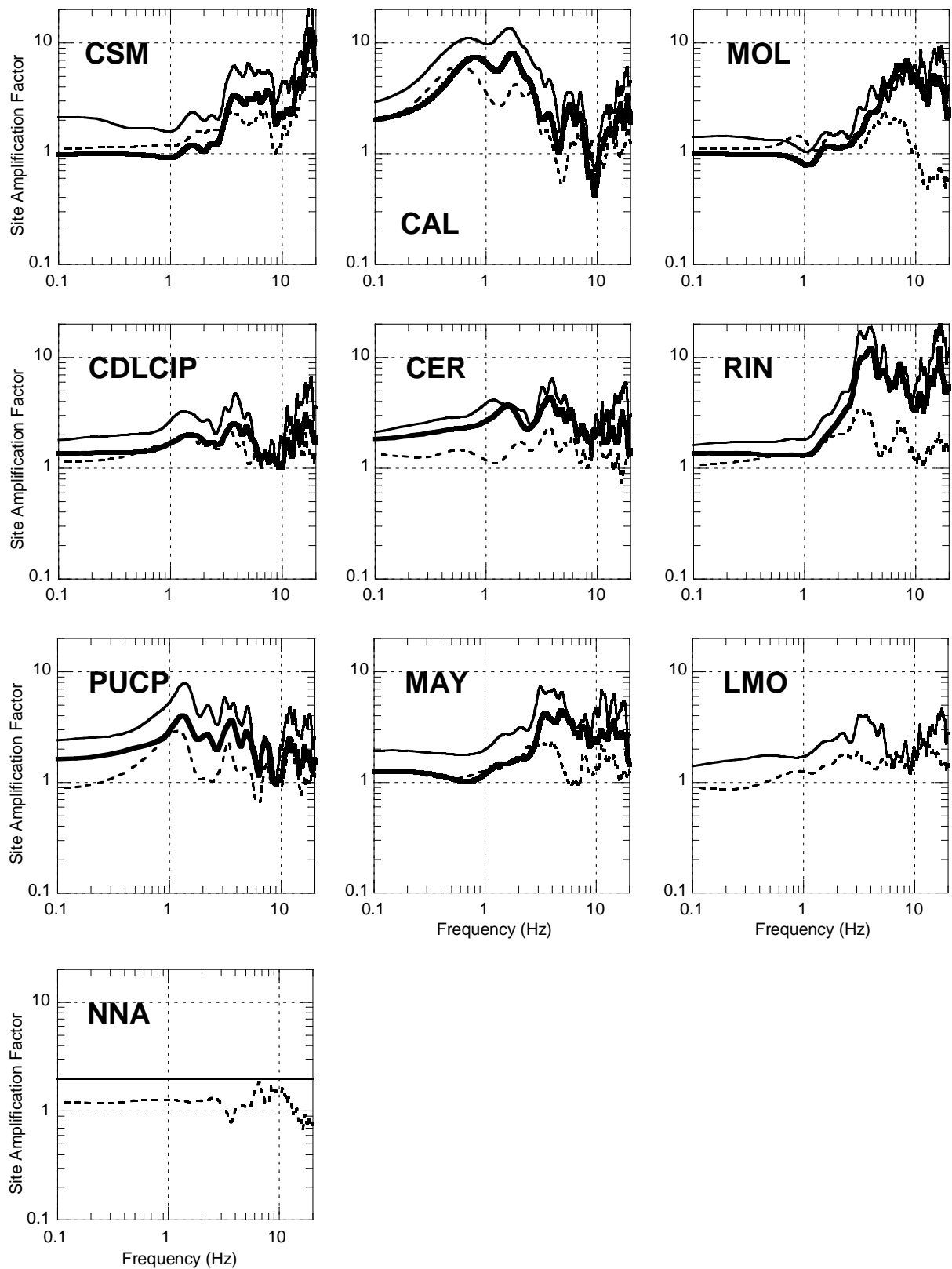
Figure 3.1. Comparison between spectral ratios from the horizontal components with reference to NNA, the Spectral Inversion Method and the Horizontal-to-Vertical Spectral Ratio. Thick solid lines show the geometrical average of two horizontal spectral ratios. Thin solid lines represent the results obtained by the Spectral Inversion Method. Dotted lines show the geometrical average estimated by applying the HVSR.
