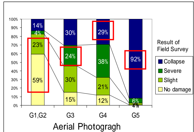
Fig.9: User's accuracy of aerial photo interpretation in central Pisco.
