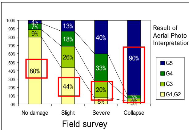
Fig.8: Producer's accuracy of aerial photo interpretation in central Pisco.
