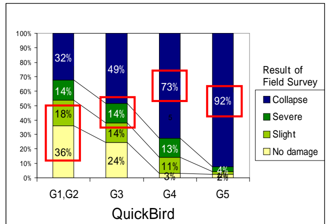
Fig. 7: User's accuracy of QB image interpretation in central Pisco.
