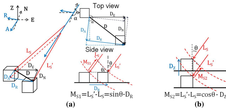
Fig.5 Schematic views of the horizontal (a) and vertical displacements (b) in a SAR image.
