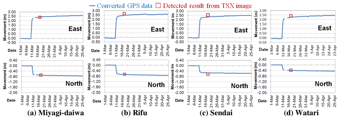
Fig. 6 Comparison of movements converted from GPS data at Miyagidaiwa (a), Rifu (b), Sendai (c), and Watari (d) ground control stations and the results detected in surrounding 25 \text{ km}^2 sub-areas.
