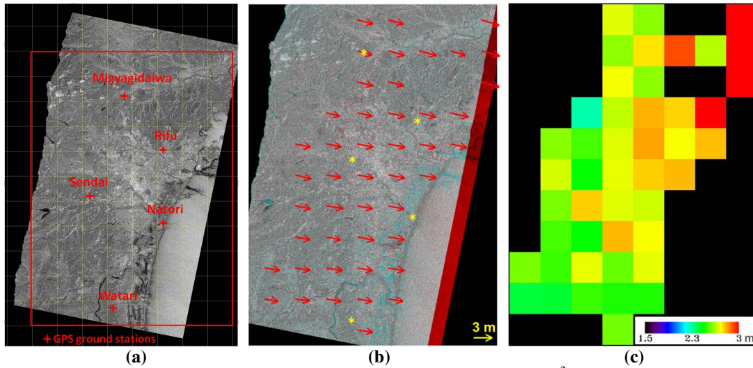
Fig. 4. Target area including 5 GPS ground station was divided into 5 \times 5 \text{ km}^2 sub-areas (a); the detected displacement vectors in each sub-area in the periods of Oct. 26, 2010 to March 18, 2011 overlapping on the color composite of the TSX intensity images (b), and the displacement amplitude values shown in rainbow color (c).
