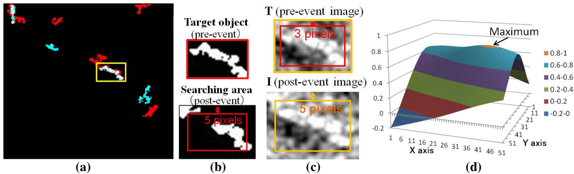
Fig. 3. A pick-up of the area in the yellow frame of Fig. 2(b) (a); a target building object in the pre-event and the search area in the post-event building image (b); target area T in the pre-event SAR image and the search area I surrounding the target area in the post-event image (c), and similarity matrix for them (d).
