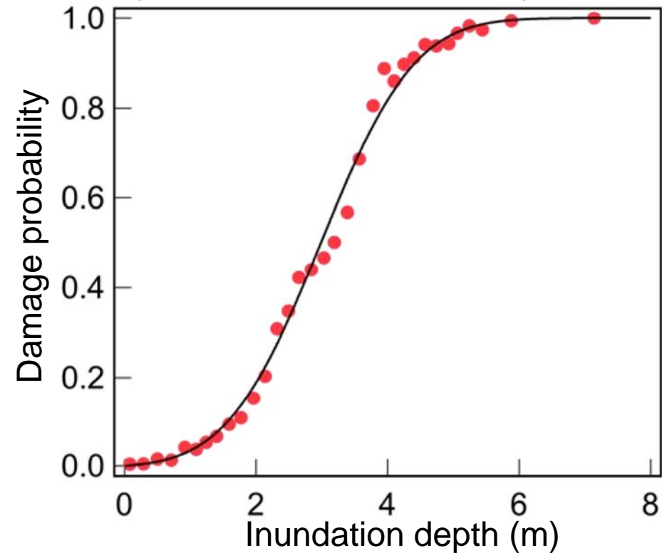
Tsunami fragility curve (Koshimura et al., 2009)
